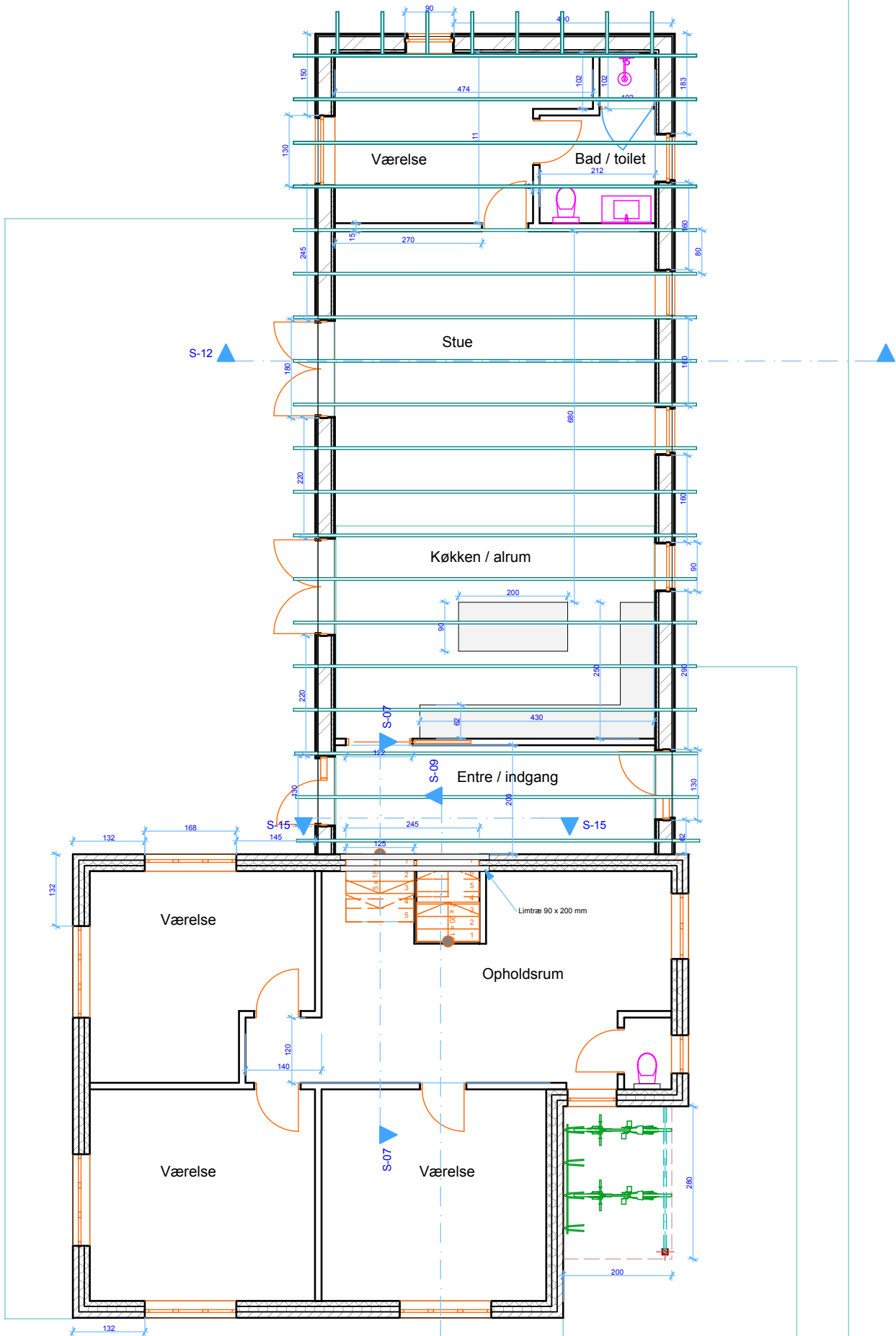
0. Ground Floor 1:100
