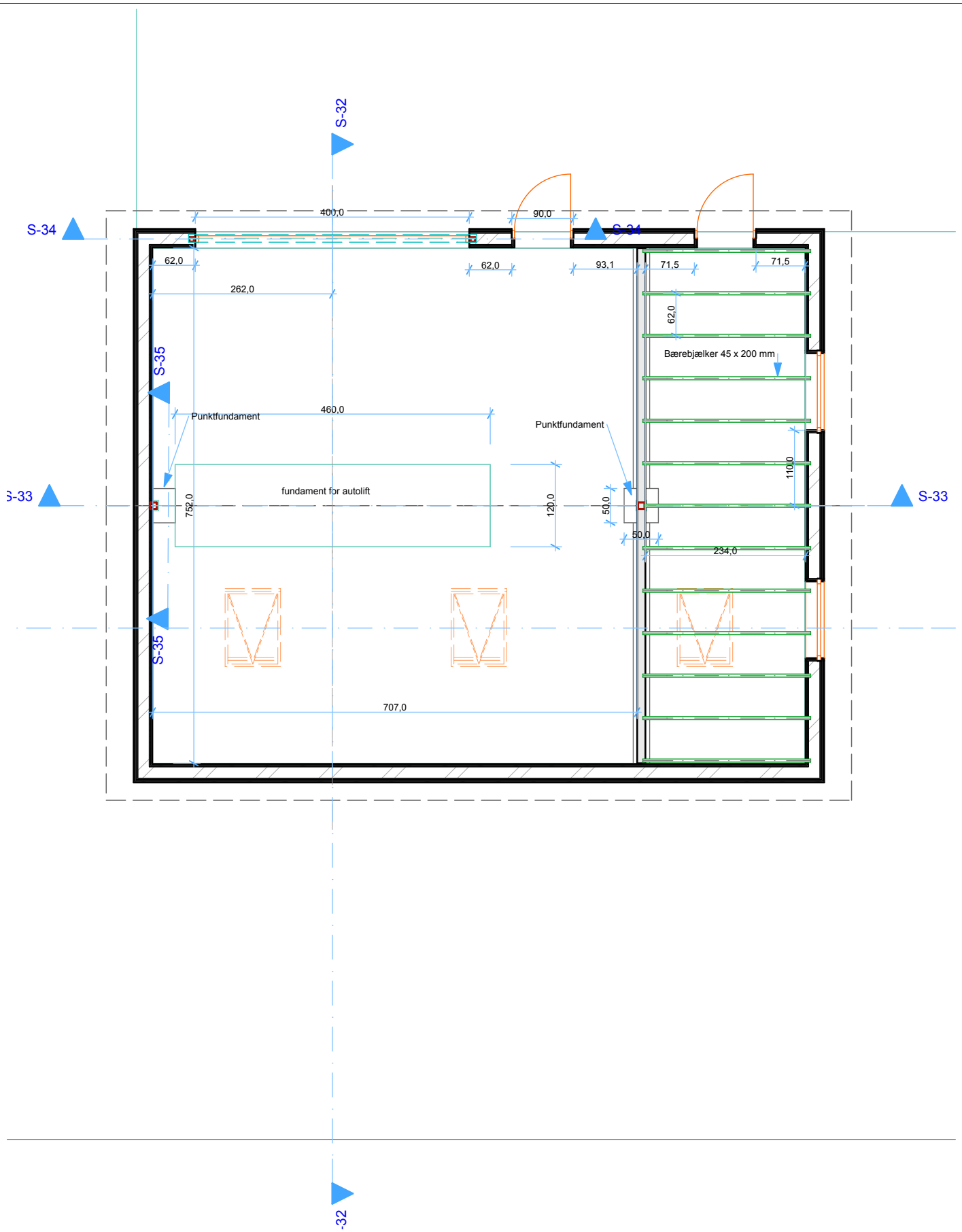
0. Ground Floor 1:75
