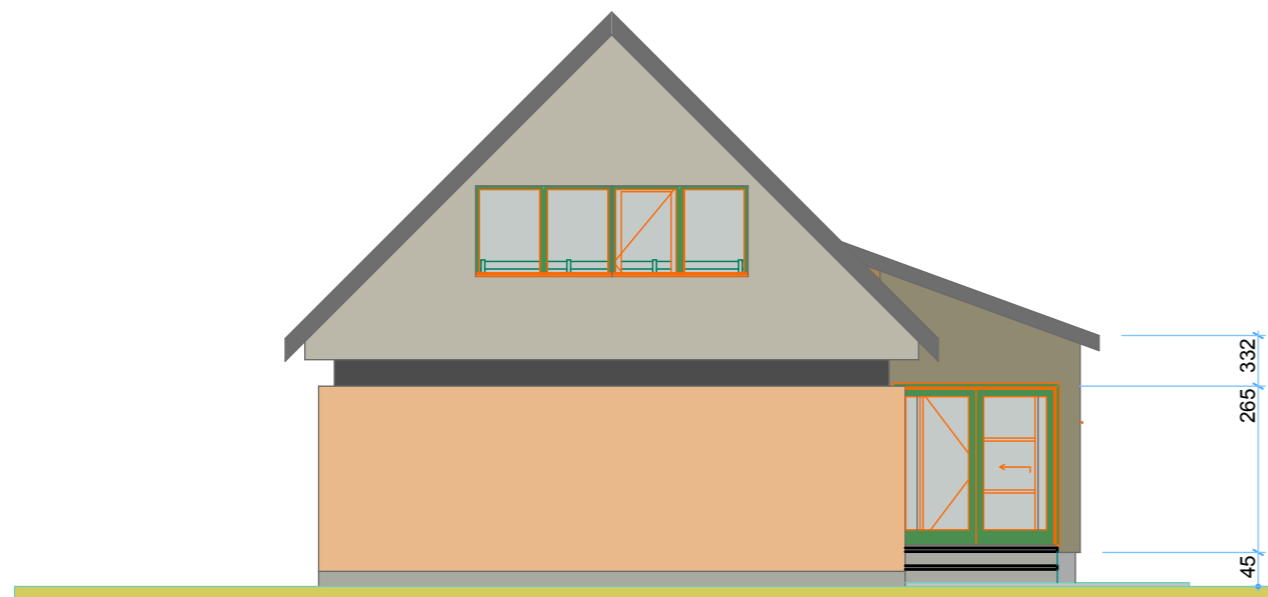
1 North Elevation 1:100
