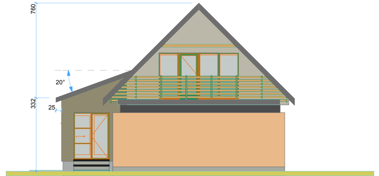
3 South Elevation 1:100
